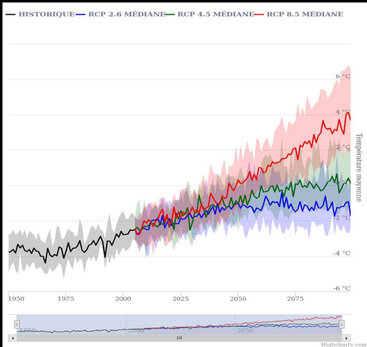
Chart 1: Historical and Projection of Mean Temperatures, 1950 to 2100, Monts Groulx (Climate Data Canada, 2019)
